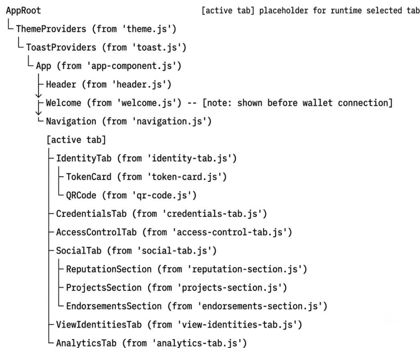
Figure 4.10 - Component Tree (§4.3.1)
