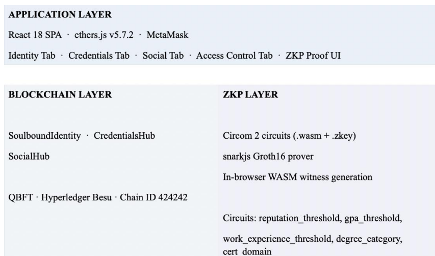
Figure 3.1 - Three-Layer Architecture (§3.1)
