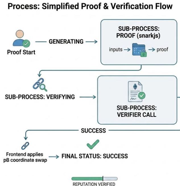
Figure 5.4- ZkpStatus State Machine (§5.5.2)
